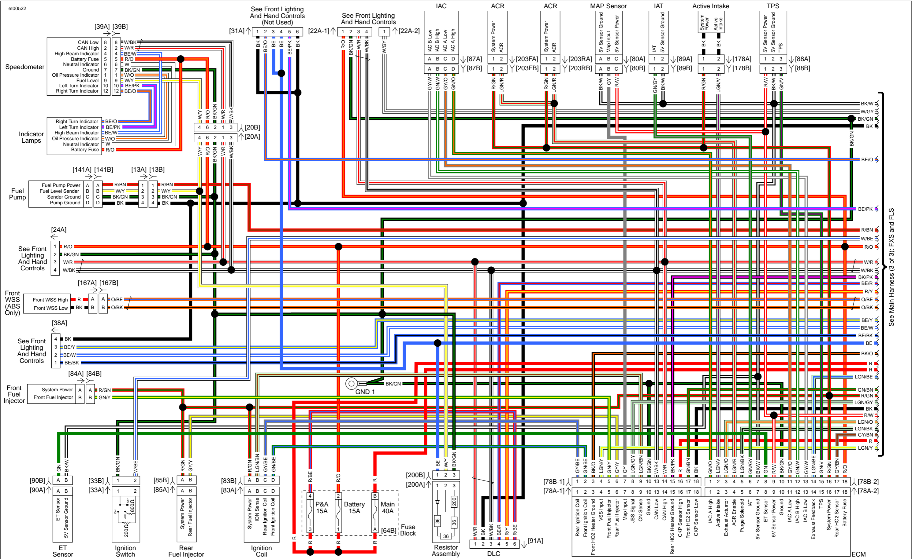
Figure B-13. Main Harness 1 of 3: 2013 Softail (FXS)
