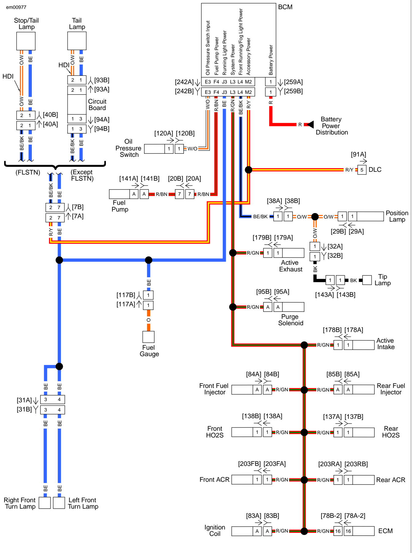
Figure B-4. Ignition and Accessory Power Distribution: Except FXS and FLS
