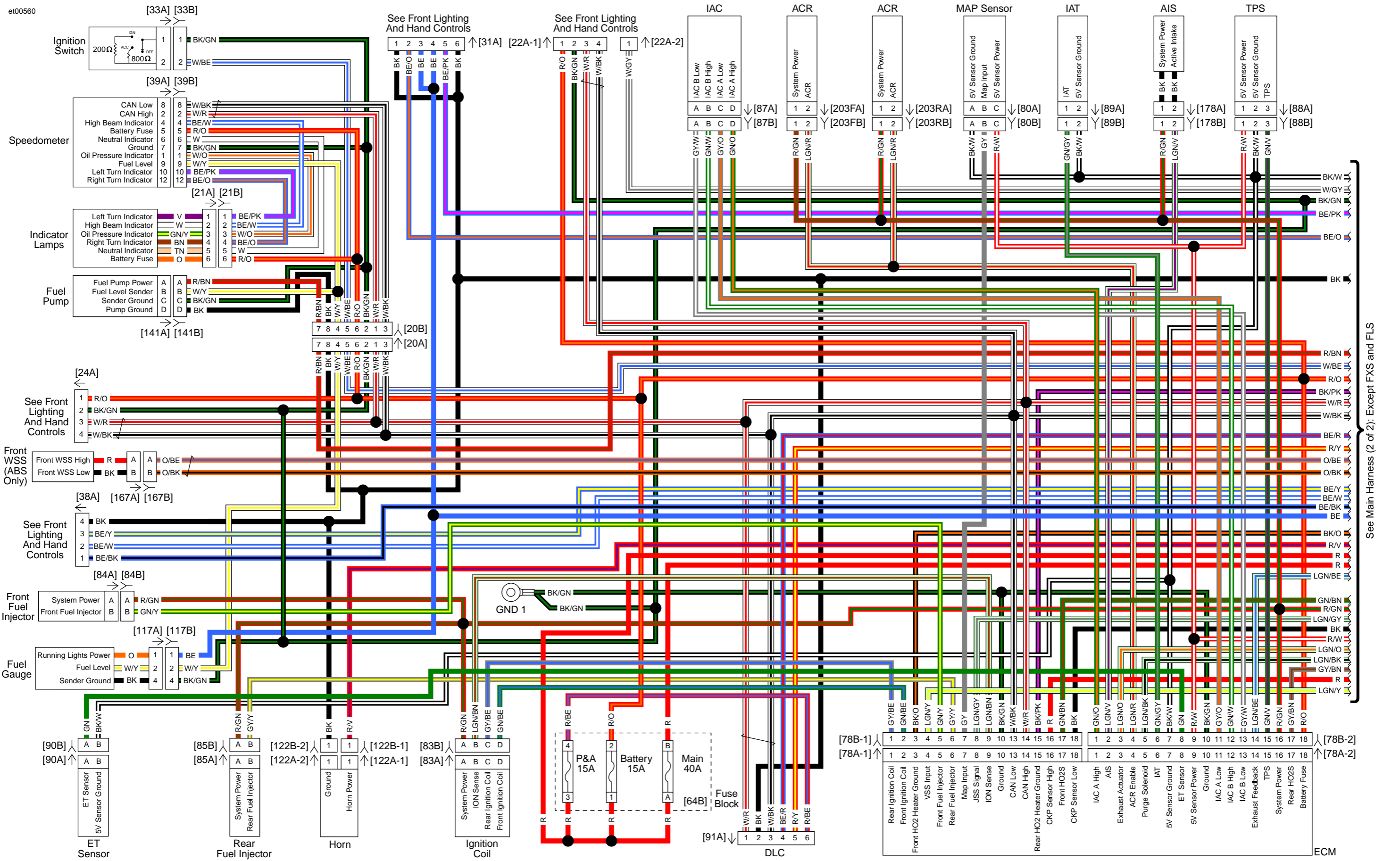
Figure B-11. Main Harness 1 of 2: 2013 Softail (Except FXS and FLS)
