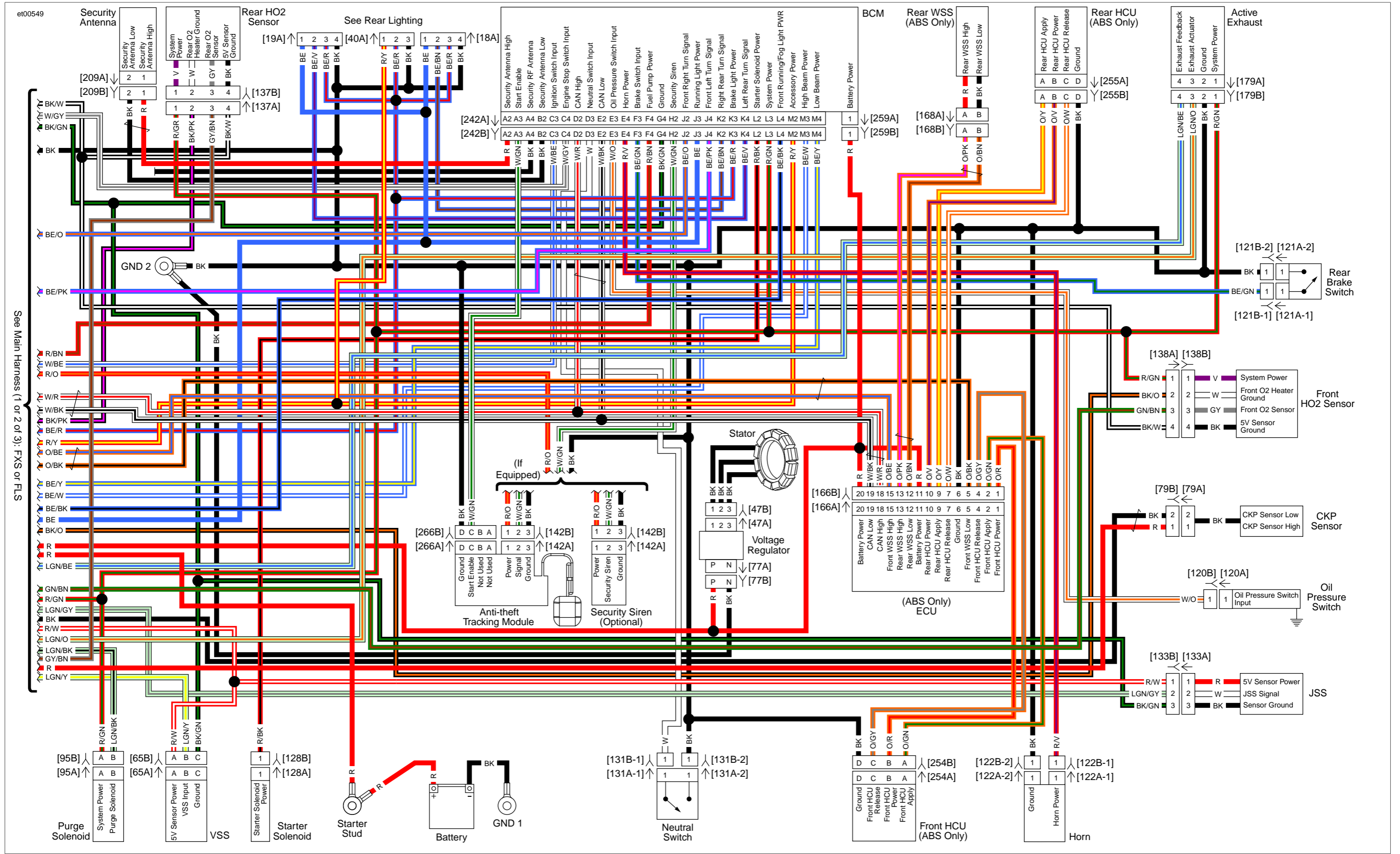
Figure B-15. Main Harness 3 of 3: 2013 Softail (FXS and FLS)
