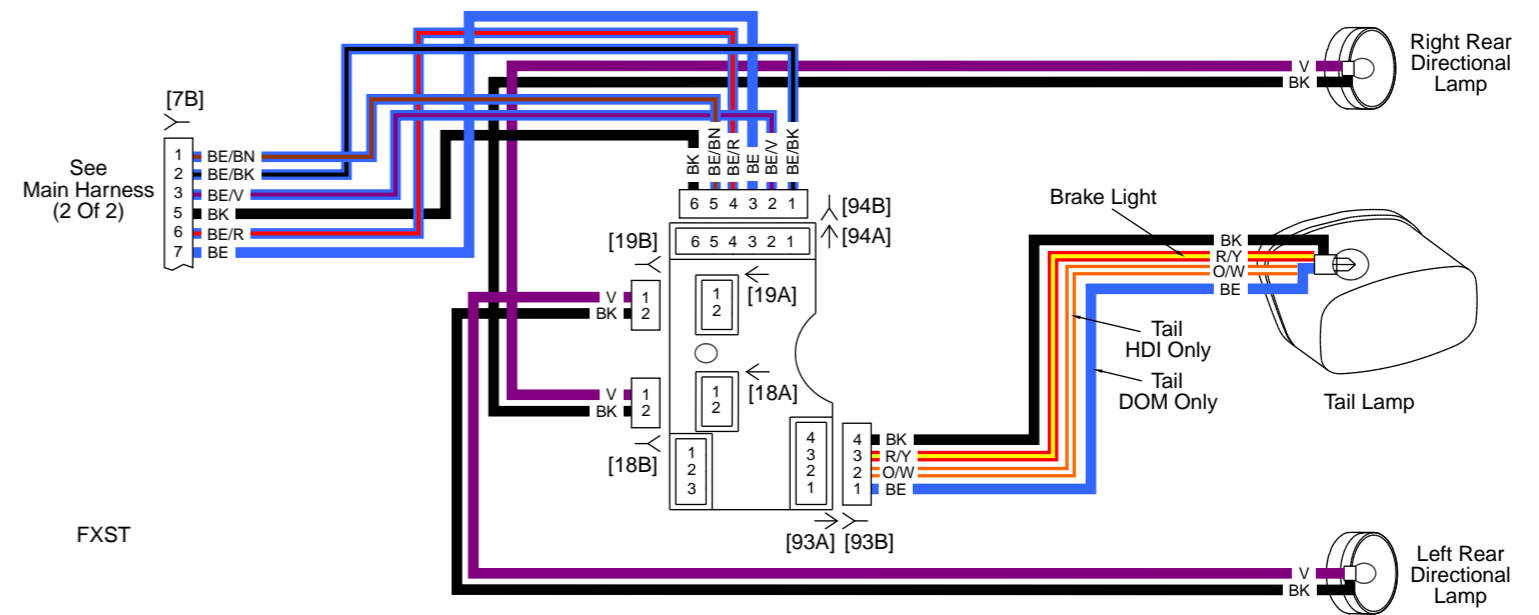
Figure B-16. Rear Lighting: 2013 Softail
