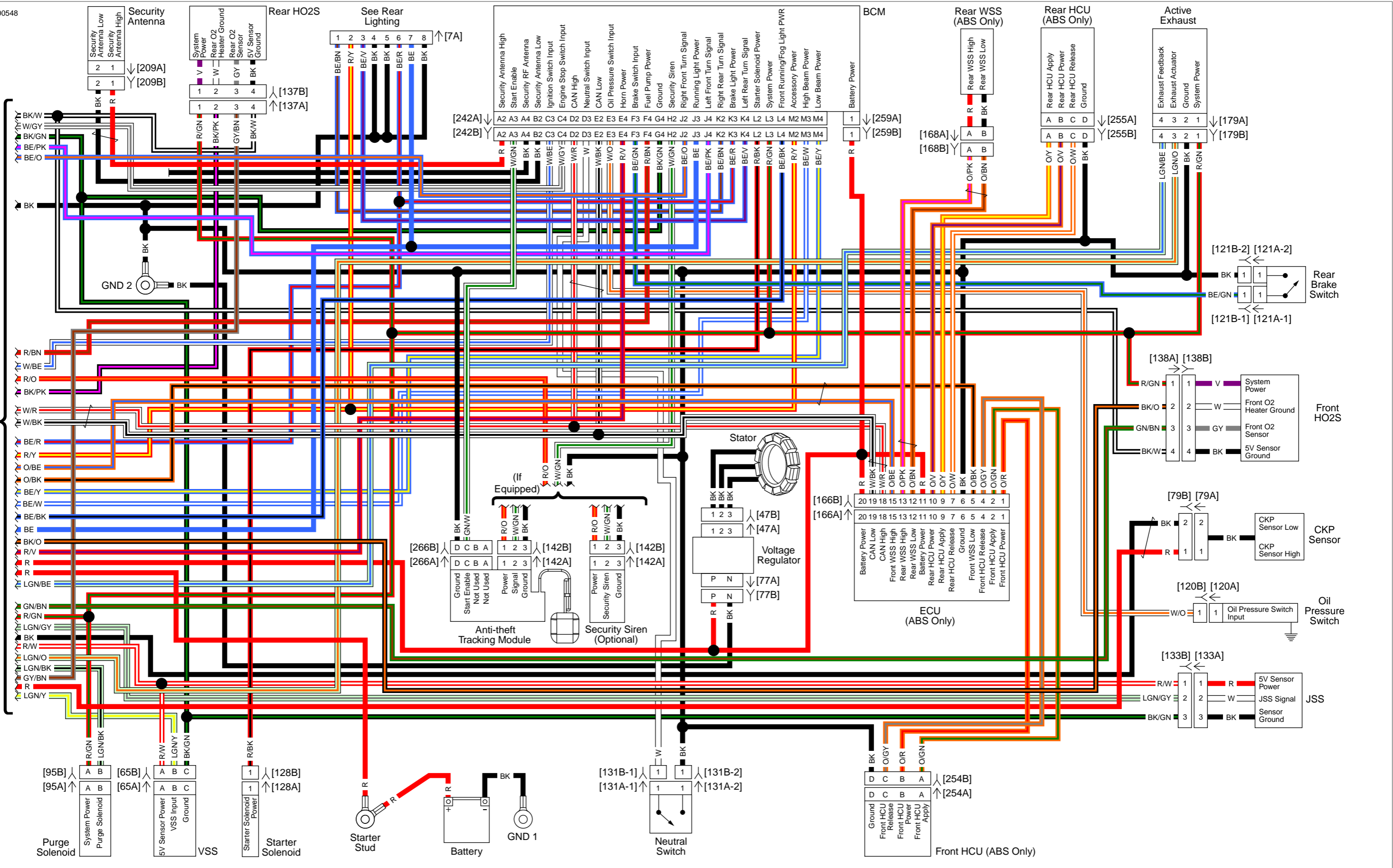
Figure B-12. Main Harness 2 of 2: 2013 Softail (Except FXS and FLS)
