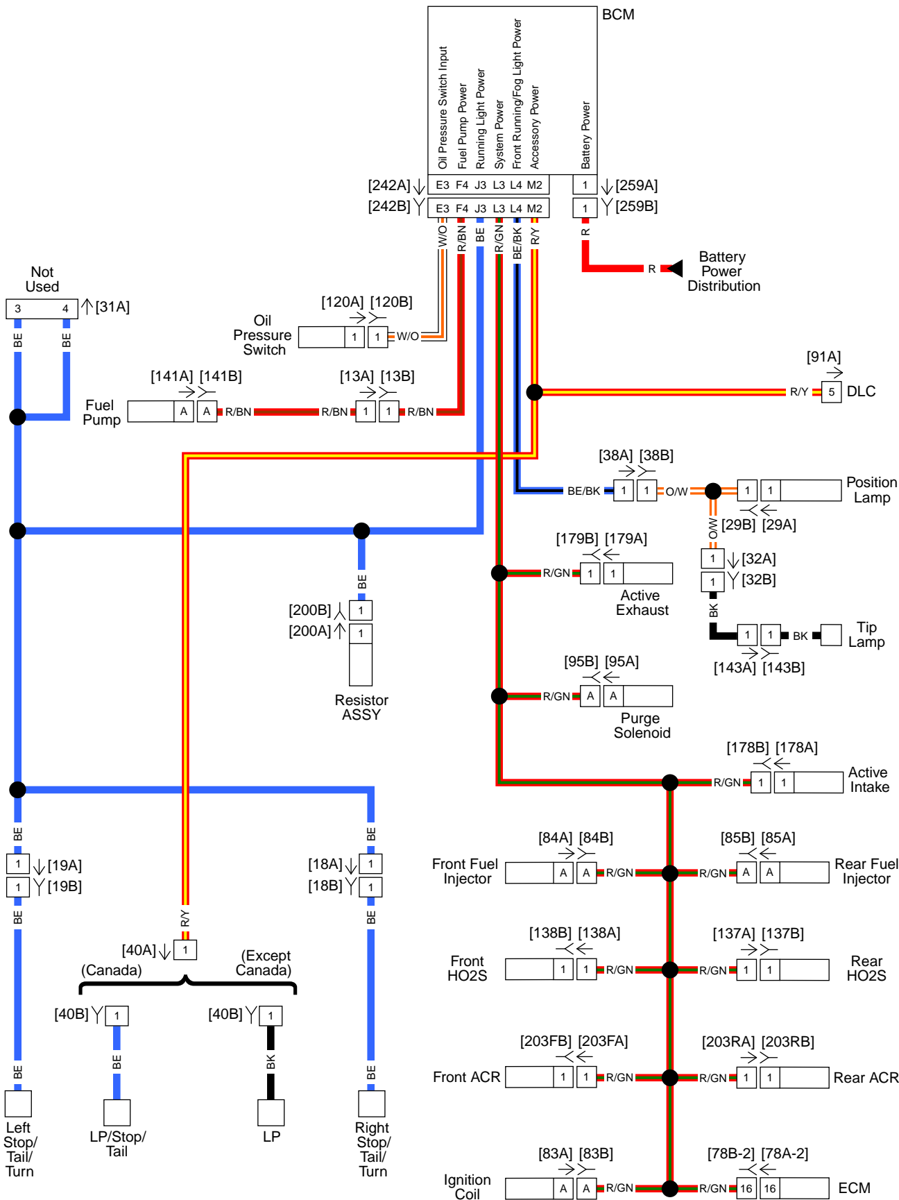
Figure B-5. Ignition and Accessory Power Distribution: FXS
