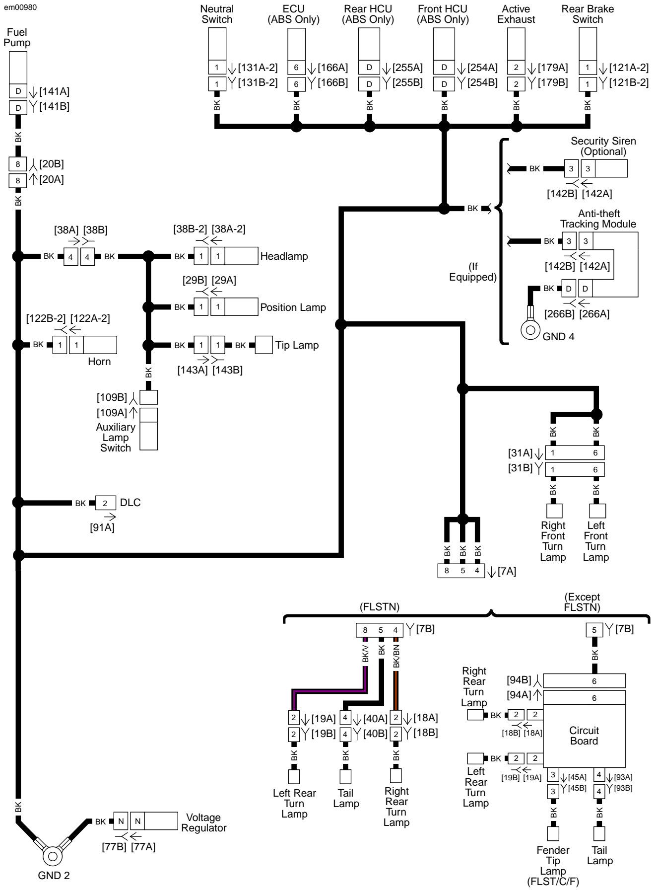
Figure B-8. Ground Circuit: Except FXS and FLS
