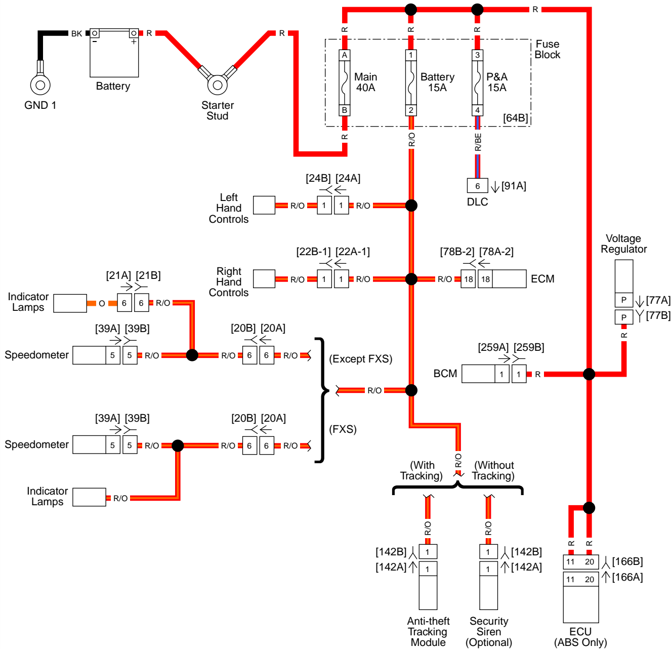
Figure B-3. Battery Power Distribution
