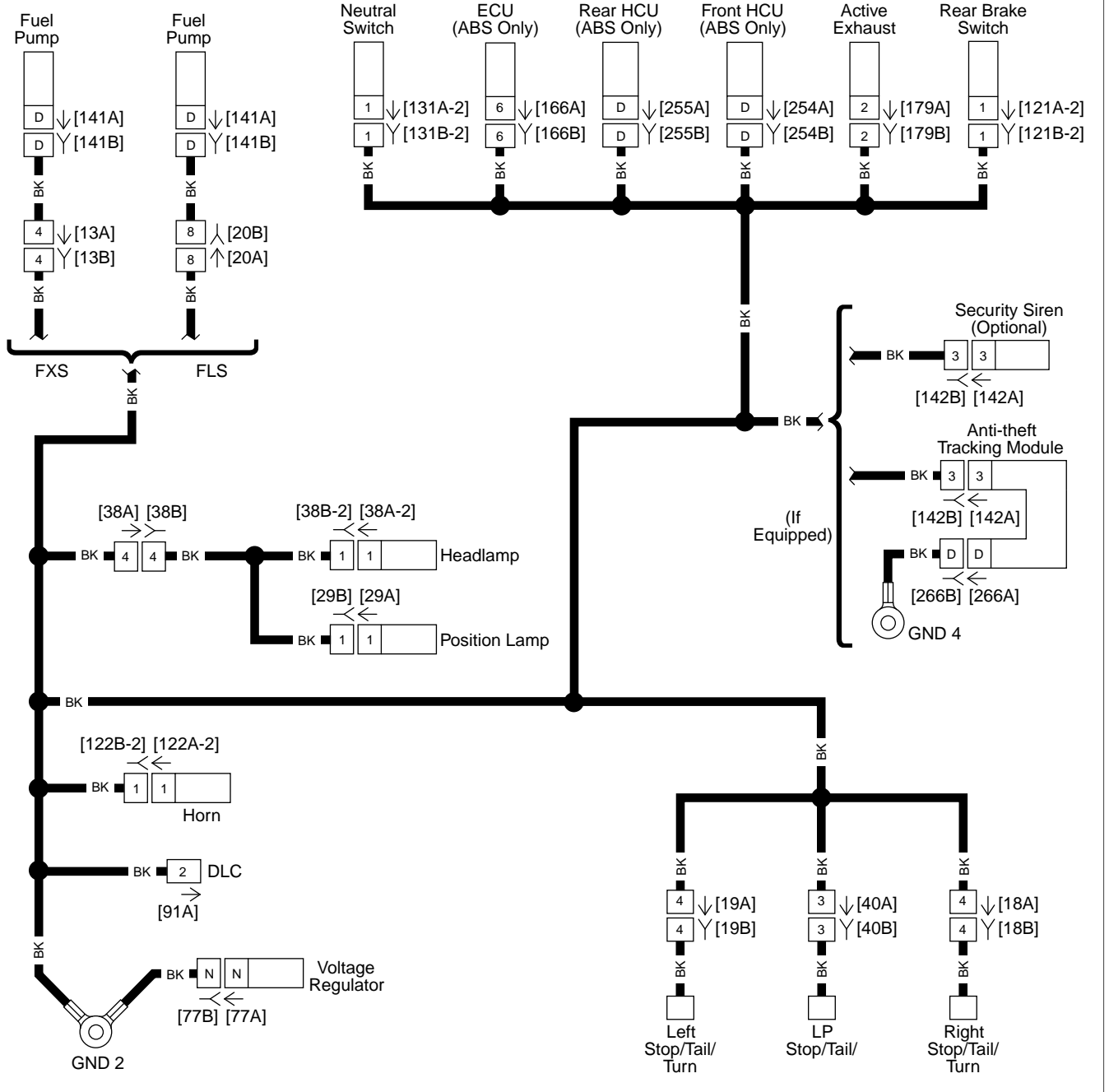
Figure B-9. Ground Circuit: FXS and FLS
