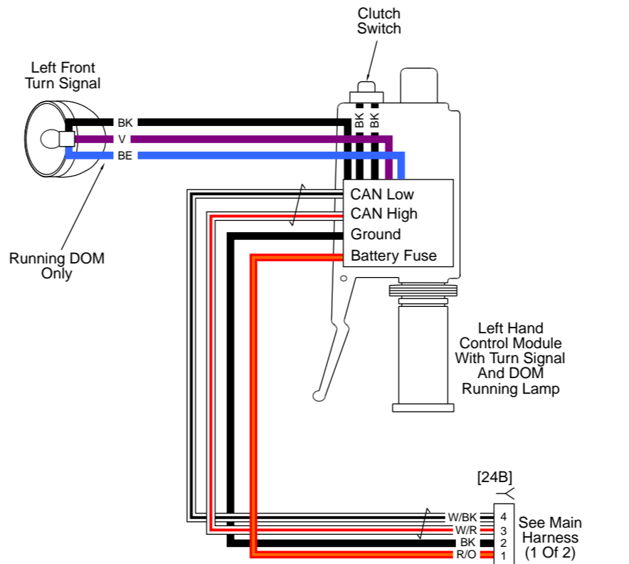
Figure B-10. Front Lighting and Hand Controls: 2013 Softail
